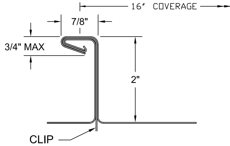
INSTALLED VIEW
