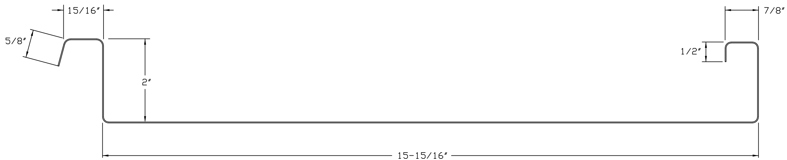
CURVED SPAN-LOK
