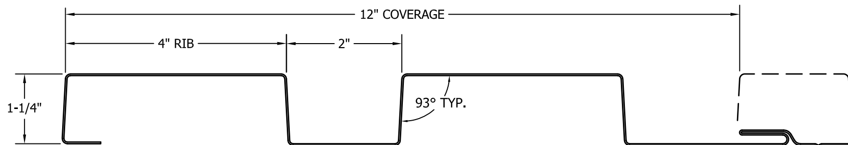
1.2FX40-12d (Direct Fastened)
