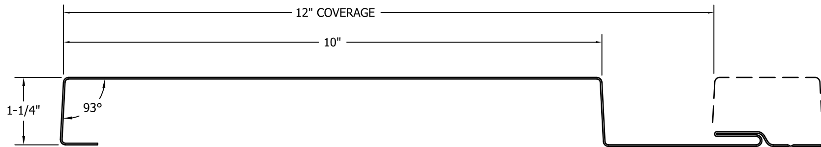
1.2FX20-12d (DIRECT FASTENED)
