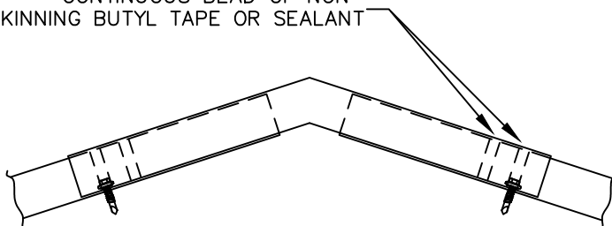
DETAIL WITH FORMED RIDGE CAP
