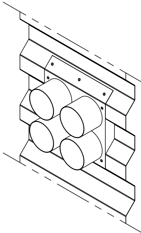
AC PIPING PENETRATION
