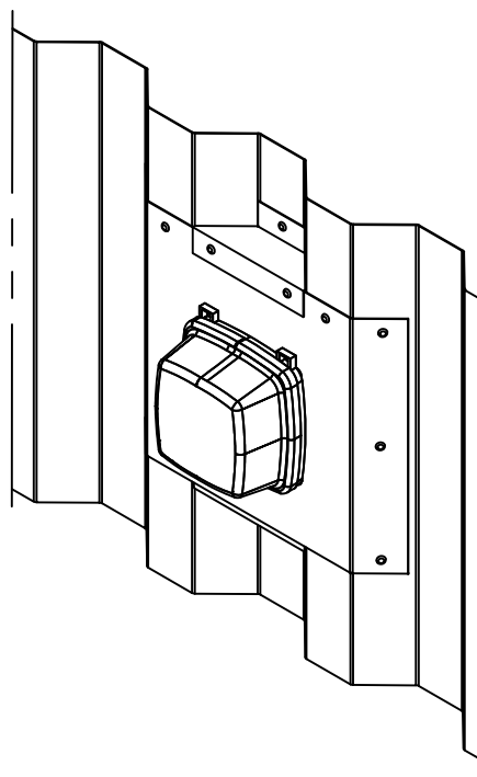
ELECTRICAL BOX PENETRATION
