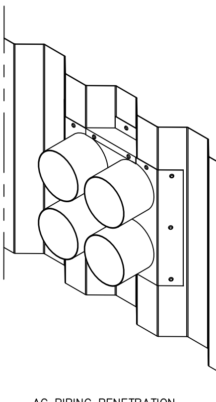
AC PIPING PENETRATION
