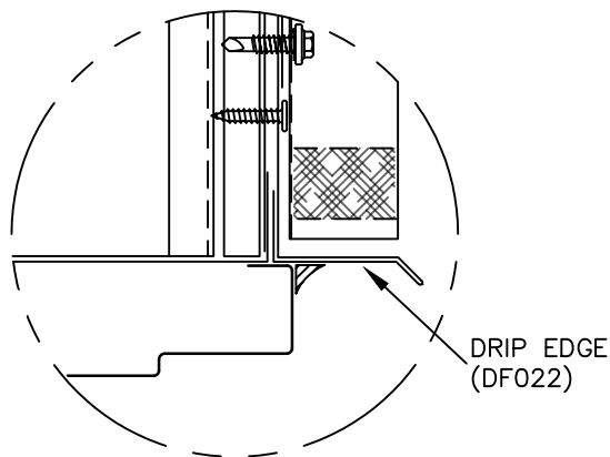
ALTERNATE DETAIL
