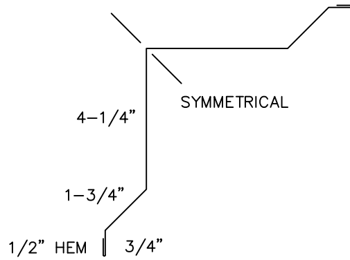
INSIDE CORNER (IC7)
