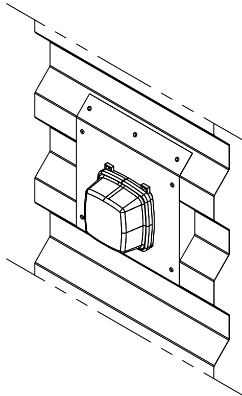
ELECTRICAL BOX PENETRATION
