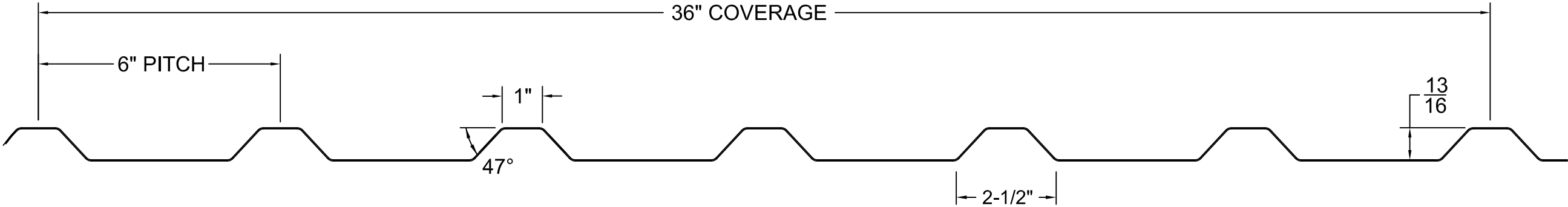
U-PANEL
